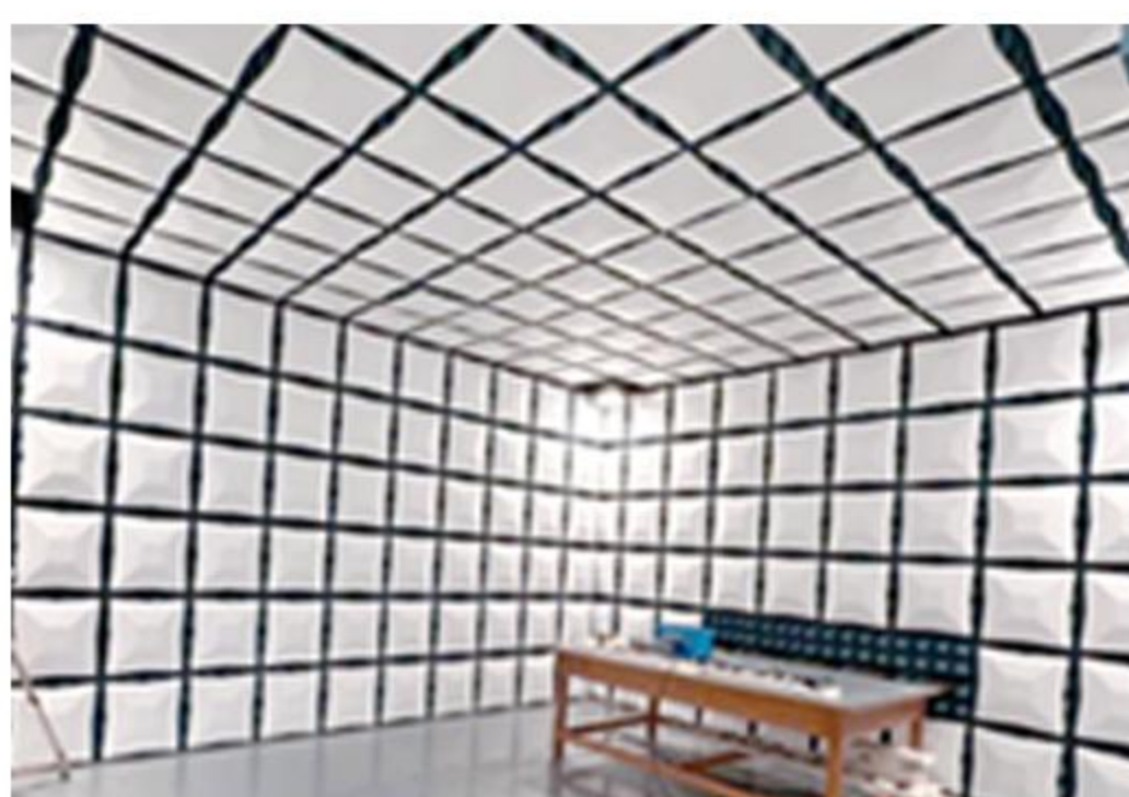
EMF test
